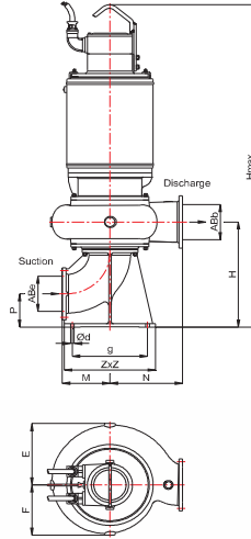
DAS-SC TYPE SUBMERSIBLE PUMP DIMENSIONS
